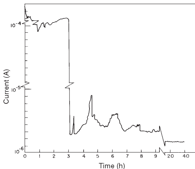
FIGURE 2. Current vs time curve for type 316L SS in 1 N HCl at applied potential of 0 \text{mV}_{\text{SCE}} .
